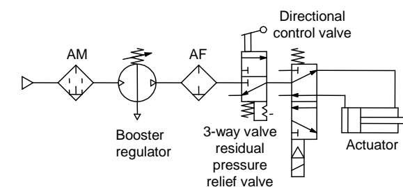
Fig.2 Circuit example (1)
