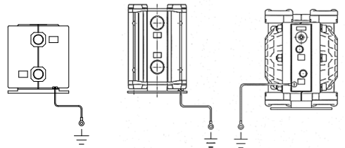
Fig.1 Method of Connecting Ground Cable *4
