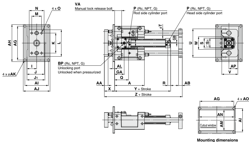
Mounting dimensions
