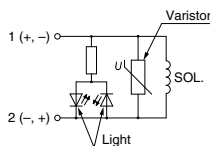
With light/surge voltage suppressor
