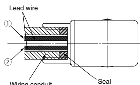
(Connection G1/2 Tightening torque 0.5 to 0.6 N·m)
