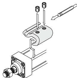
(ø32 D-P3DWA取付例)
