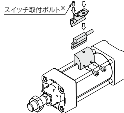
(ø32 D-P3DWA取付例)
